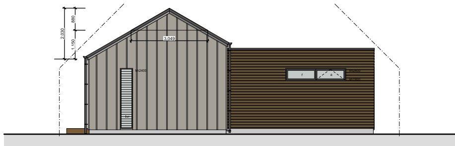
Concept South Elevation Scale: 1:50
