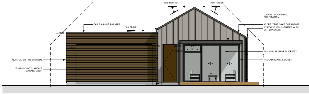
Concept North Elevation Scale: 1:50
